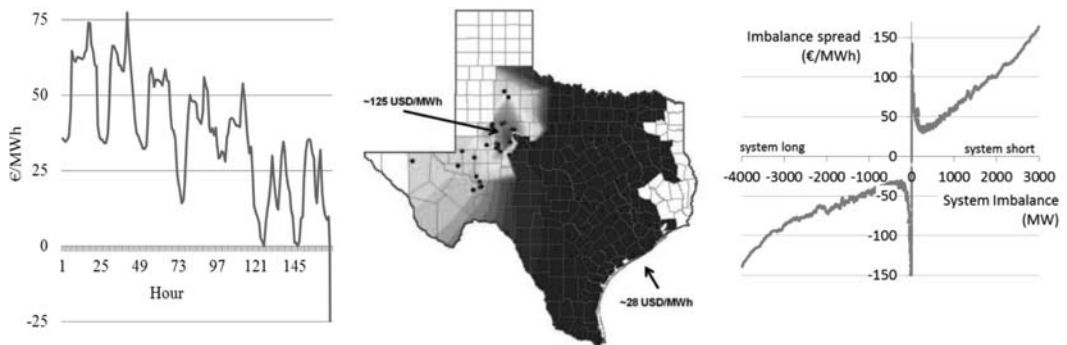
Figure 1: Observed Electricity Prices in Germany and Texas
