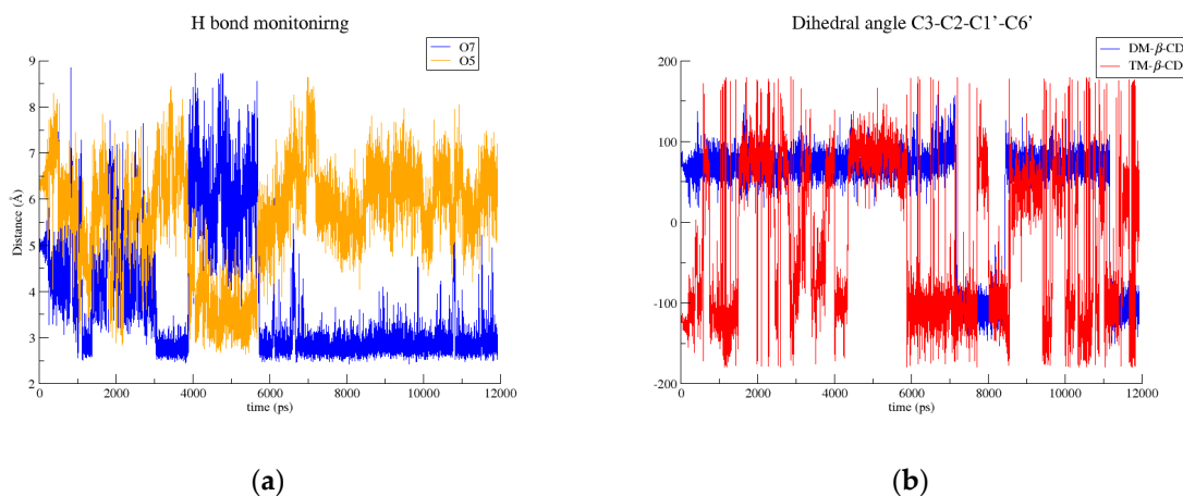
Figure 6. (a) H-bond monitoring between the hydroxyls of the ring A of the chromone group (atoms O7 and O5) of the guest molecule and the secondary methoxy group of the third glucose unit of TM- \beta -CD and (b) dihedral angle C3-C2-C1'-C6' of naringenin in both hosts.
