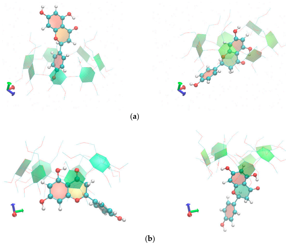
Figure 5. Representative snapshots for (a) naringenin/DM- \beta -CD at: 0 ns (left) and 2 ns (right), and for (b) naringenin/TM- \beta -CD at: 0 ns (left) and 8 ns (right). Guest molecules are depicted as ball-and-stick models and hosts' macrocycle as a paperchain.
