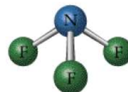
Trigonal pyramidal
