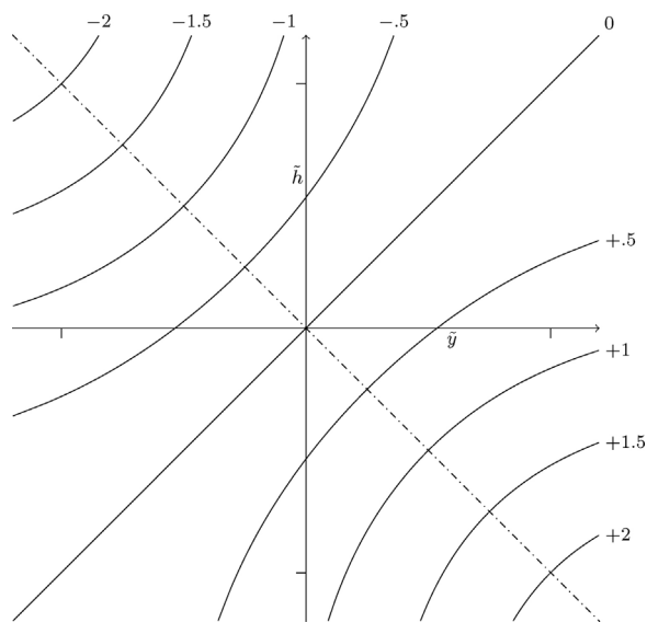
Fig. 3.2. Some equipaced levels of the index D_p , for c = 1 , in the (\tilde{y}, \tilde{h}) -plane. The symmetric green growth/brown degrowth locus is the dashed and dotted line. (Ticks are 1 unit apart on both axes.)
