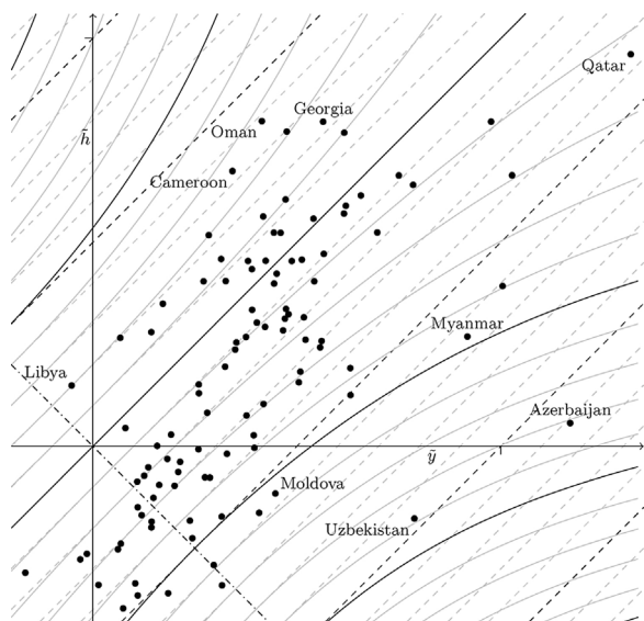
Fig. 4.1. Some equispaced levels of the indices D_N (dashed lines) and D_P for c = 1 (solid curves) in the (\tilde{y}, \tilde{h}) -plane and the data cloud of world countries for the decade 2003–2013. The symmetric green growth/brown degrowth locus is the dashed and dotted line. (Ticks are 1 unit apart on both axes.)
